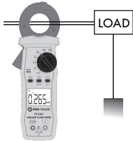
Fig. 2 Measuring out of balance leakage current:
