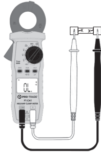
Open Circuit
